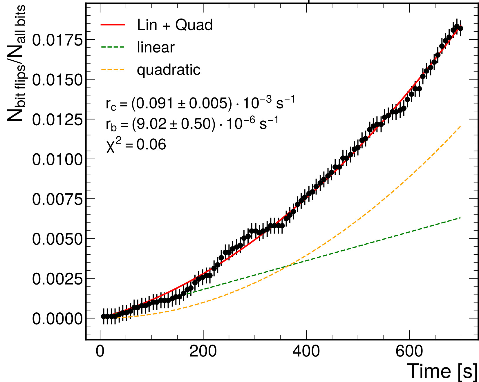
0-1 Bitflips
