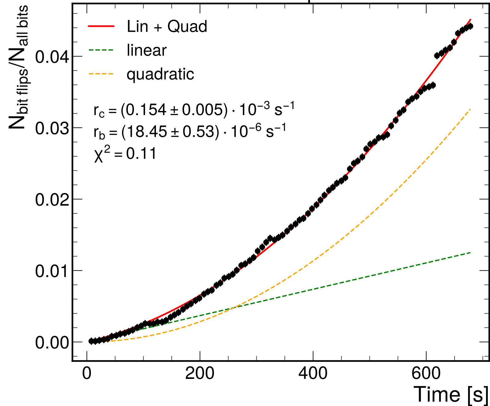
0-1 Bitflips
