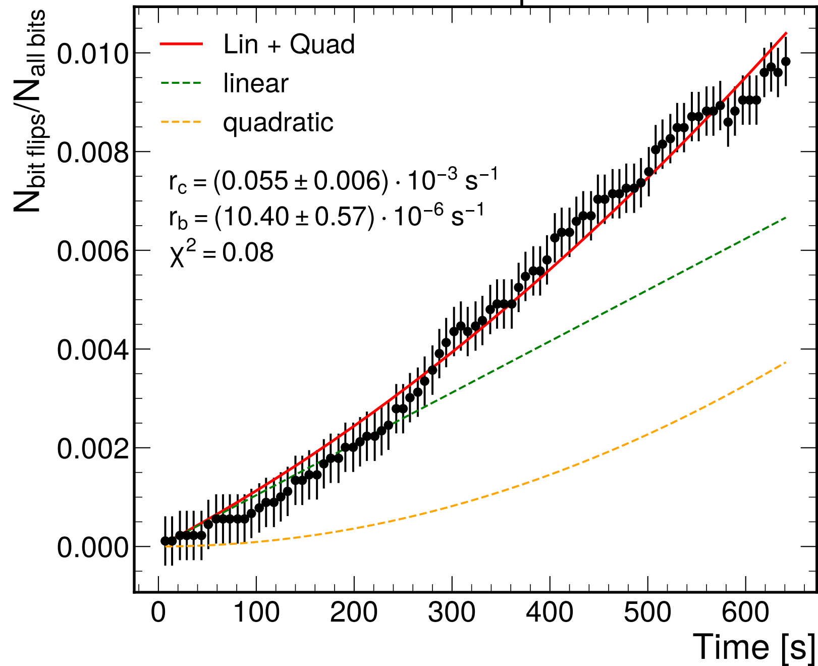
0-1 Bitflips
