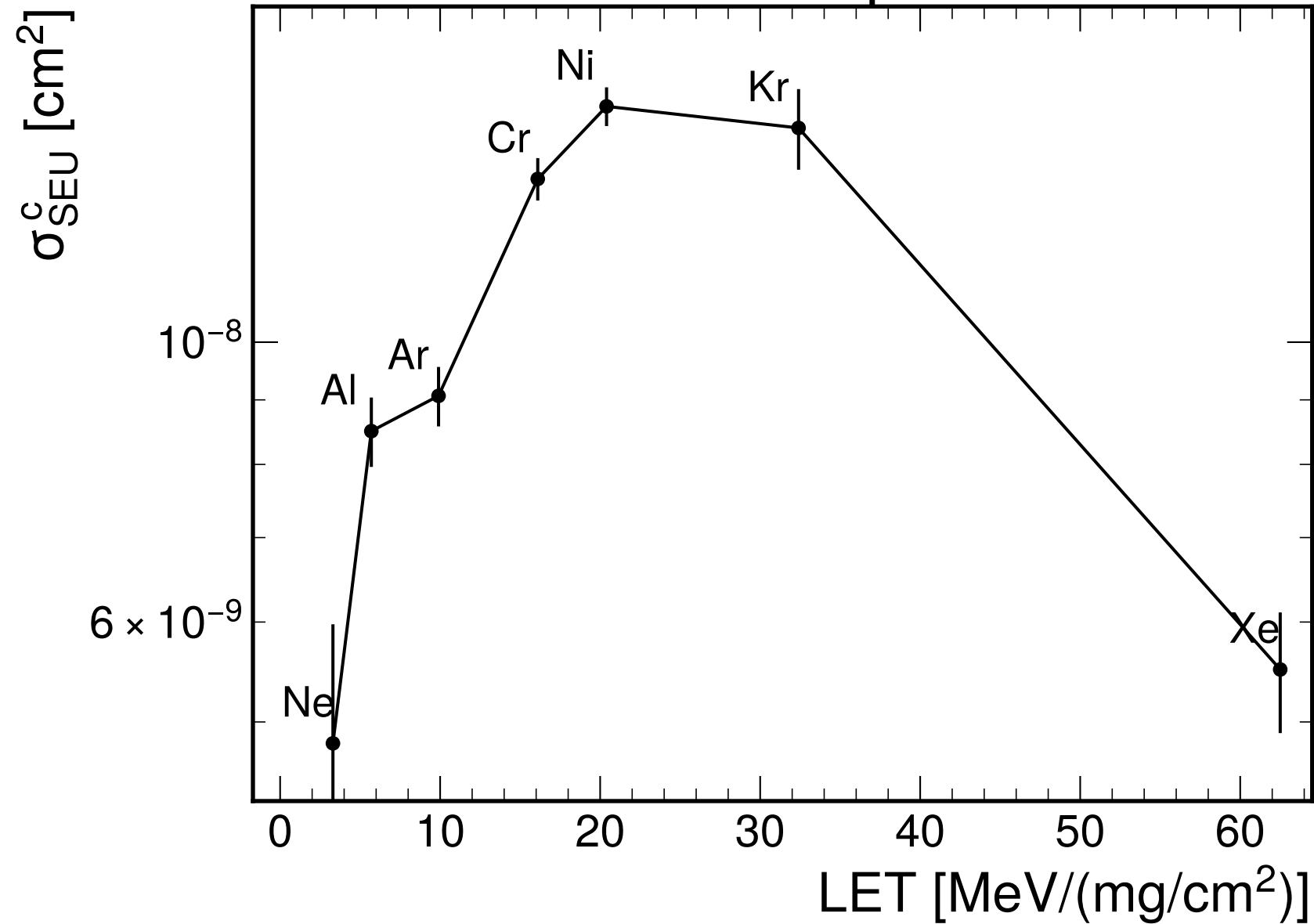
0-1 Bitflips
