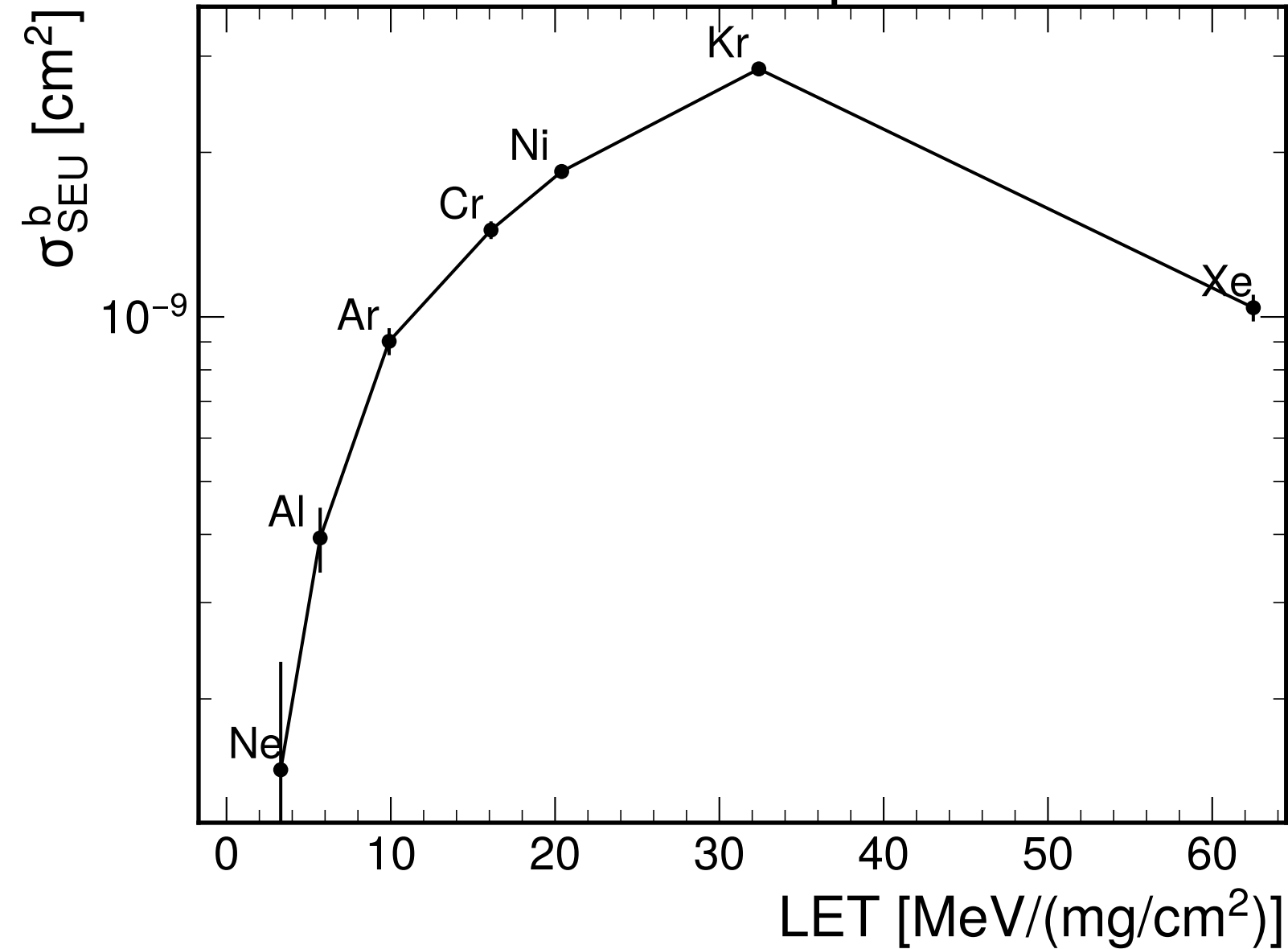
0-1 Bitflips
