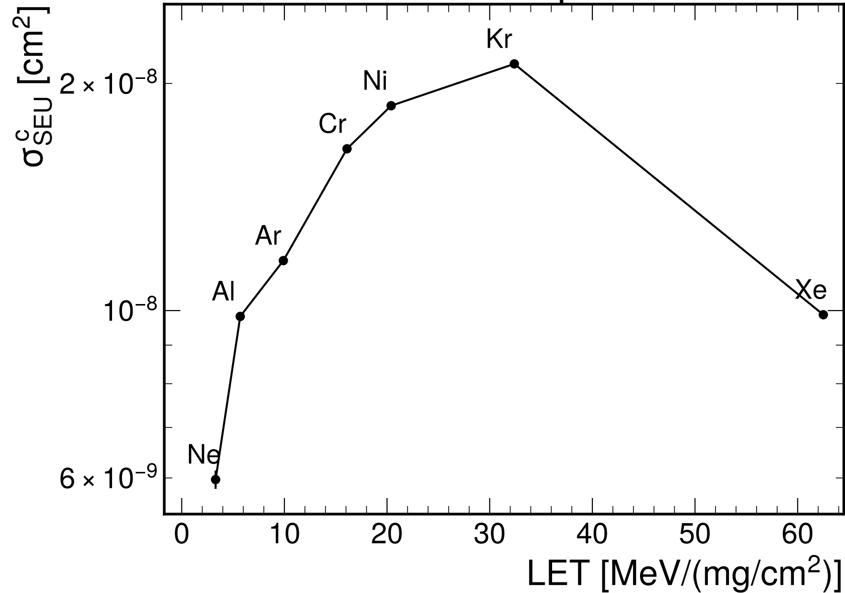
0-1 Bitflips
