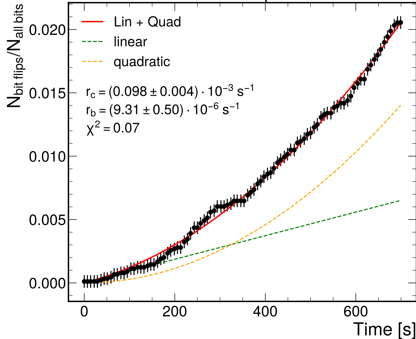
0-1 Bitflips
