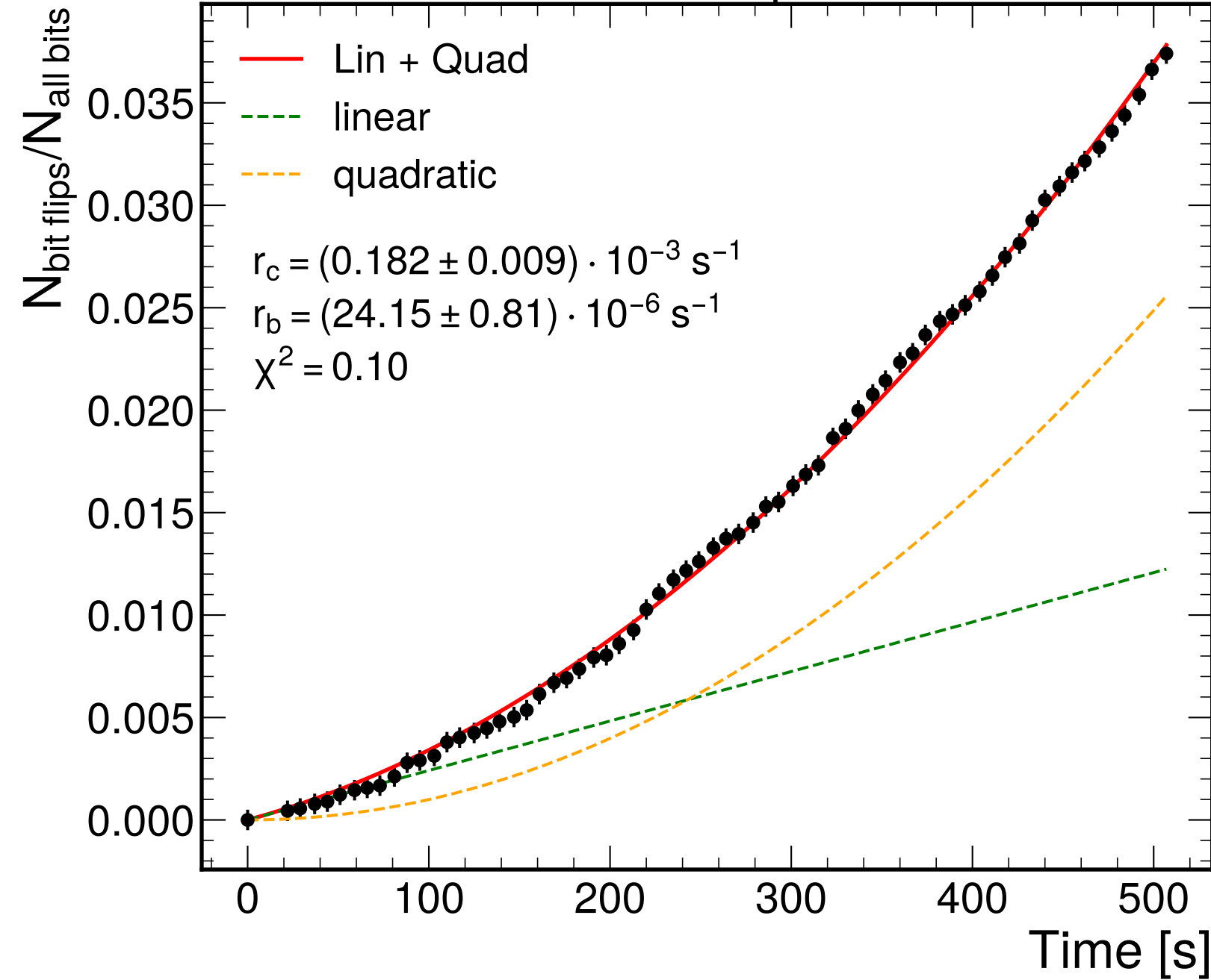
0-1 Bitflips
