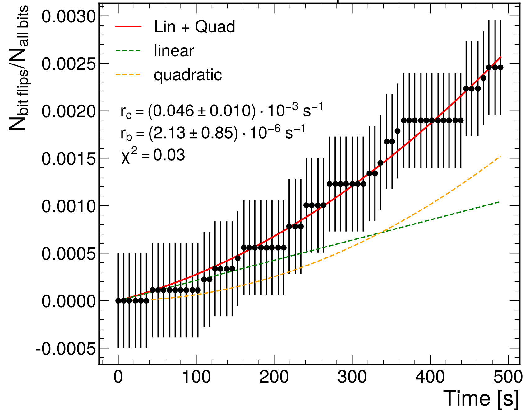
0-1 Bitflips
