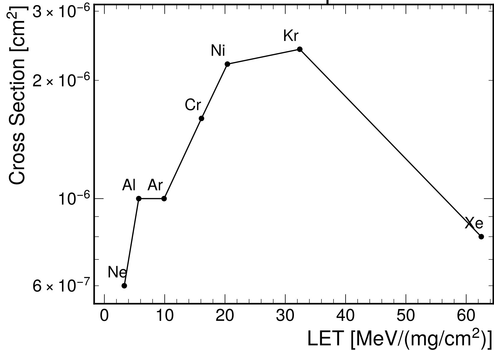
0-1 Bitflips
