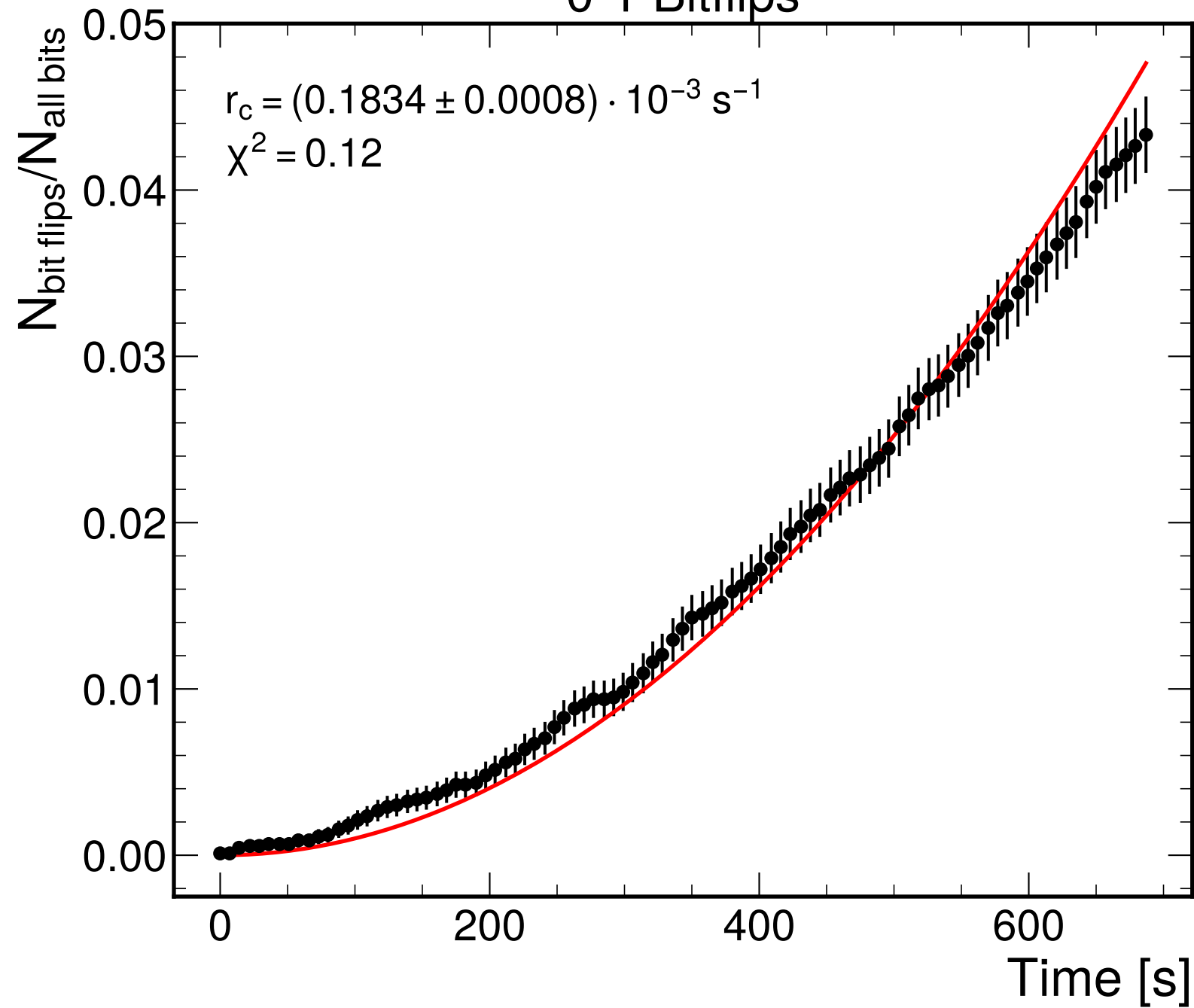
0-1 Bitflips
