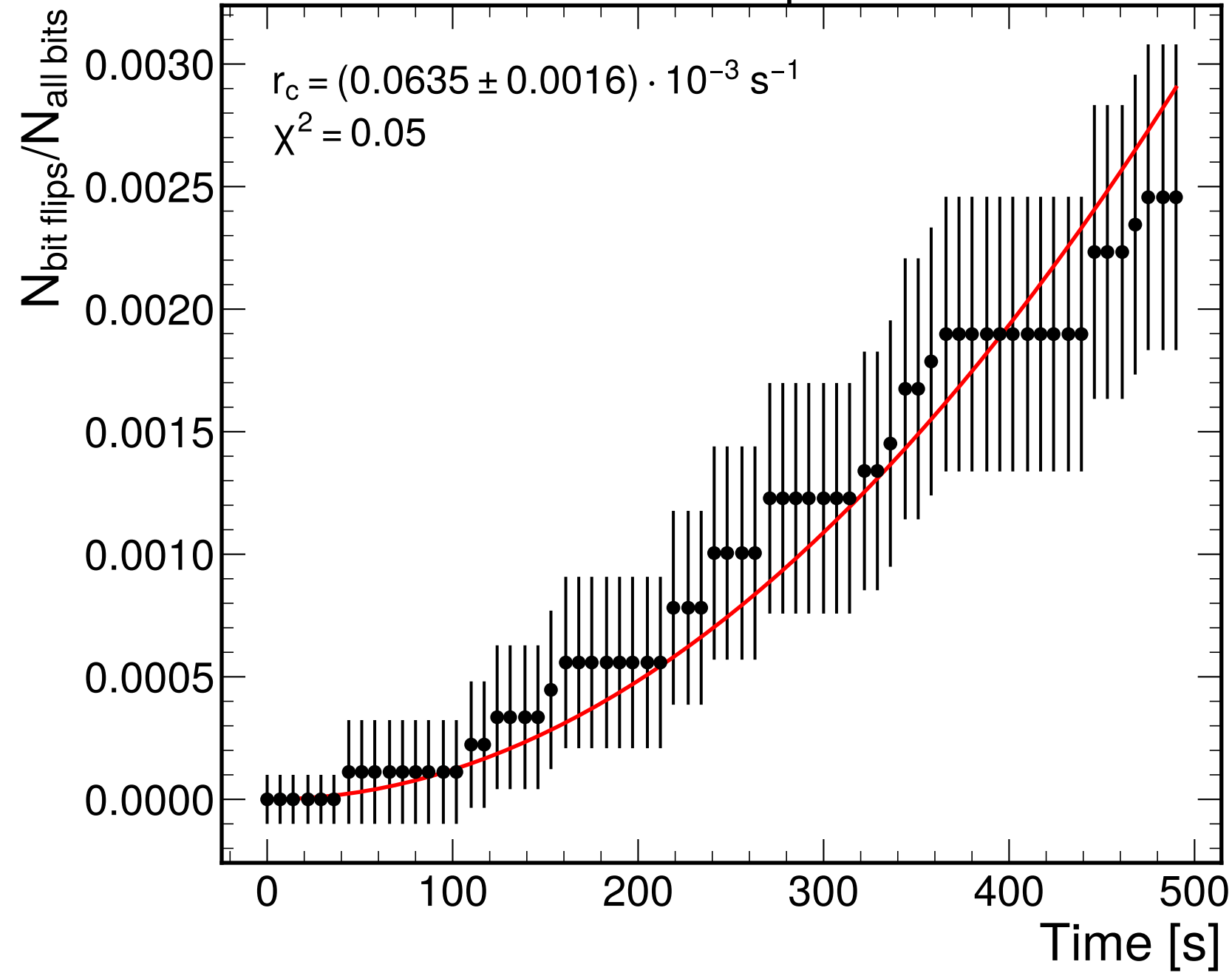
0-1 Bitflips
