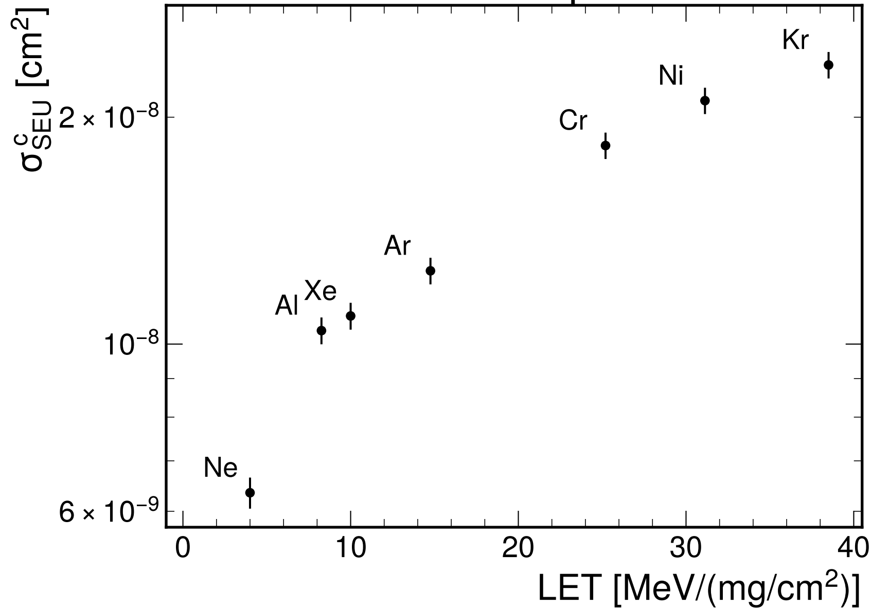
0-1 Bitflips
