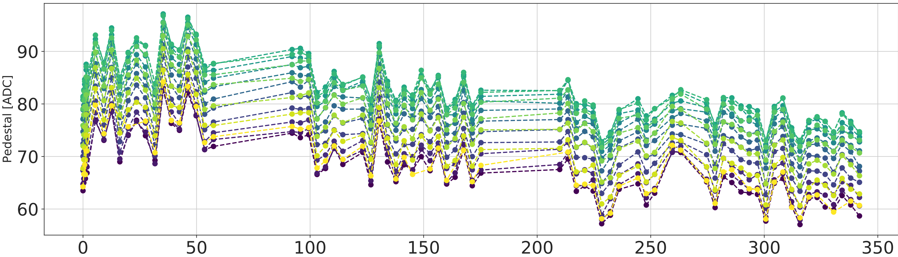
Phase Scan channel 7 Roc 002
