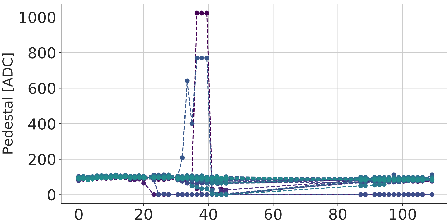
Pedestal Run measurements Roc 003
