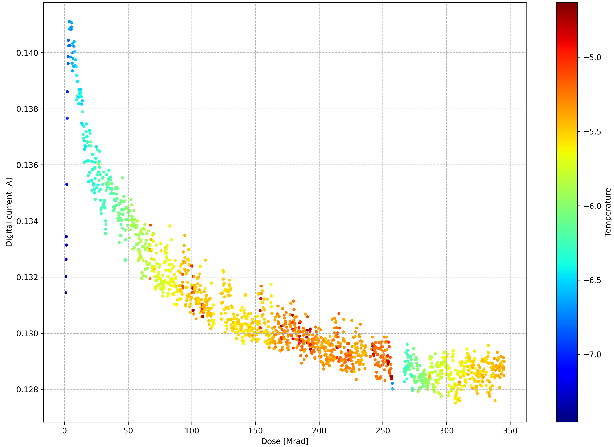
PSU Measurements
