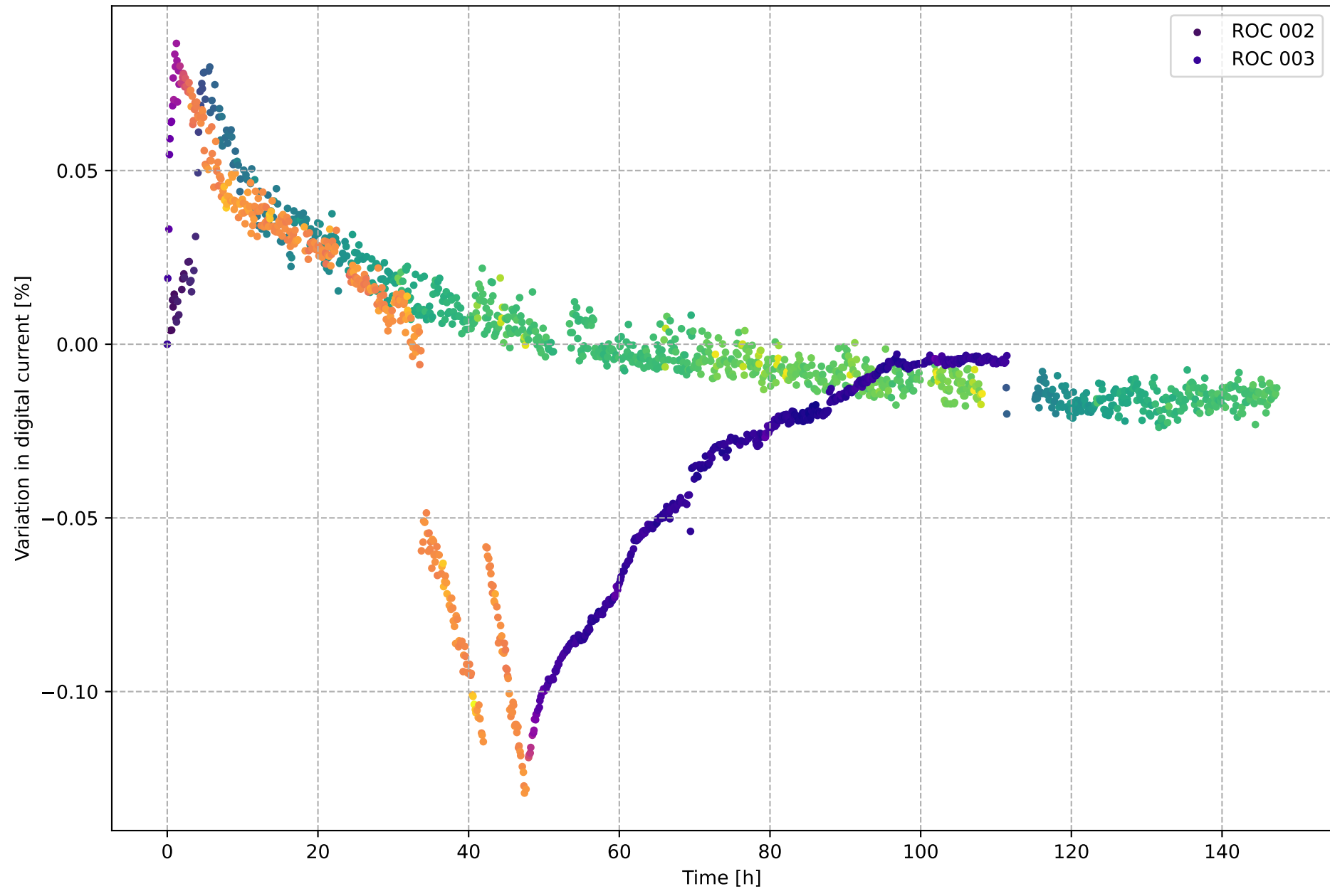
PSU Measurements
