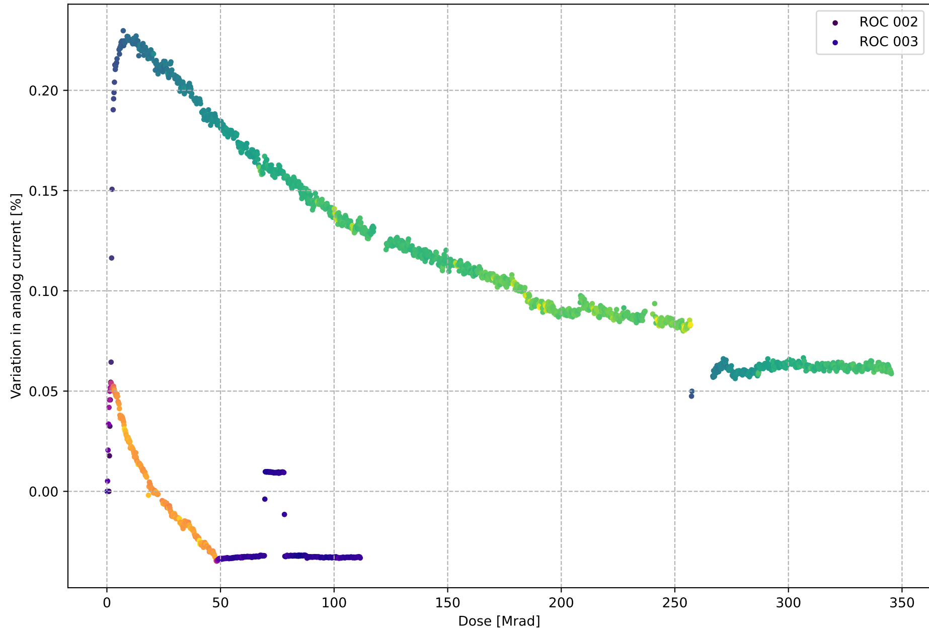
PSU Measurements
