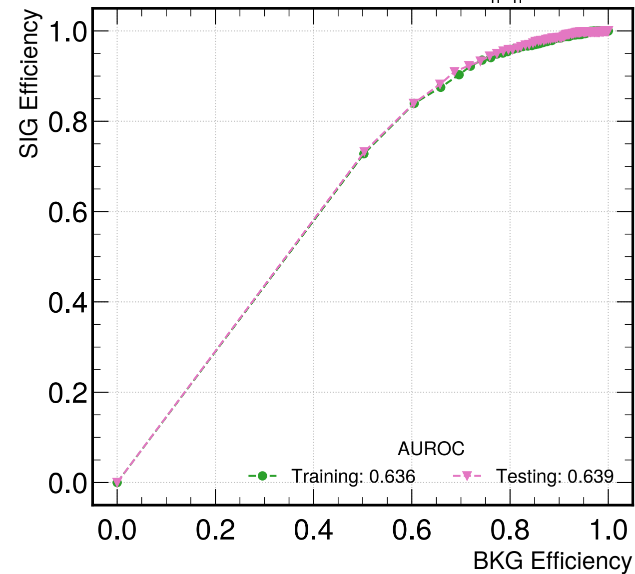
Boosted b - Resolved \tau -- \tau_h\tau_h
