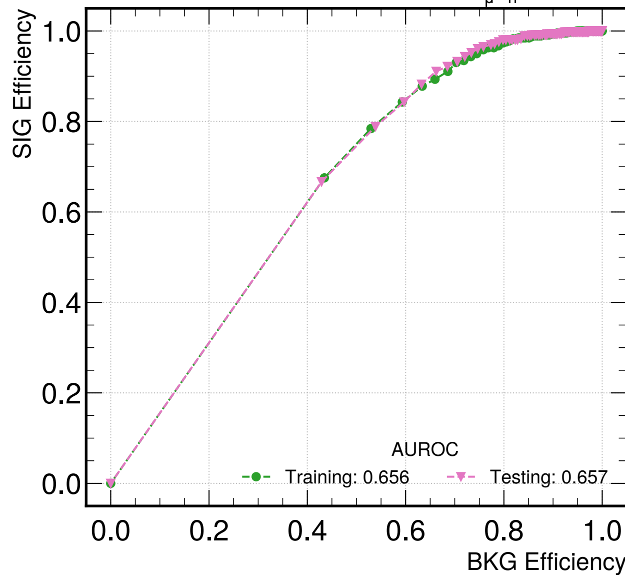
Boosted b - Resolved \tau -- \tau_\mu\tau_h
