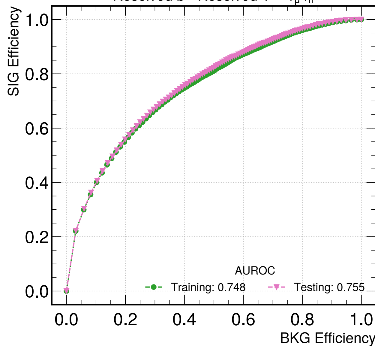
Resolved b - Resolved \tau -- \tau_\mu\tau_h
