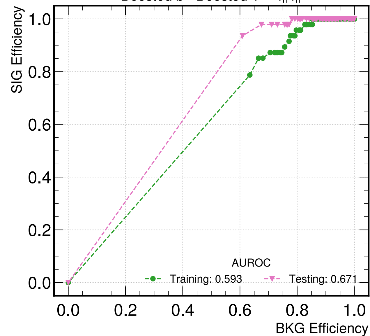
Boosted b - Boosted \tau -- \tau_h\tau_h
