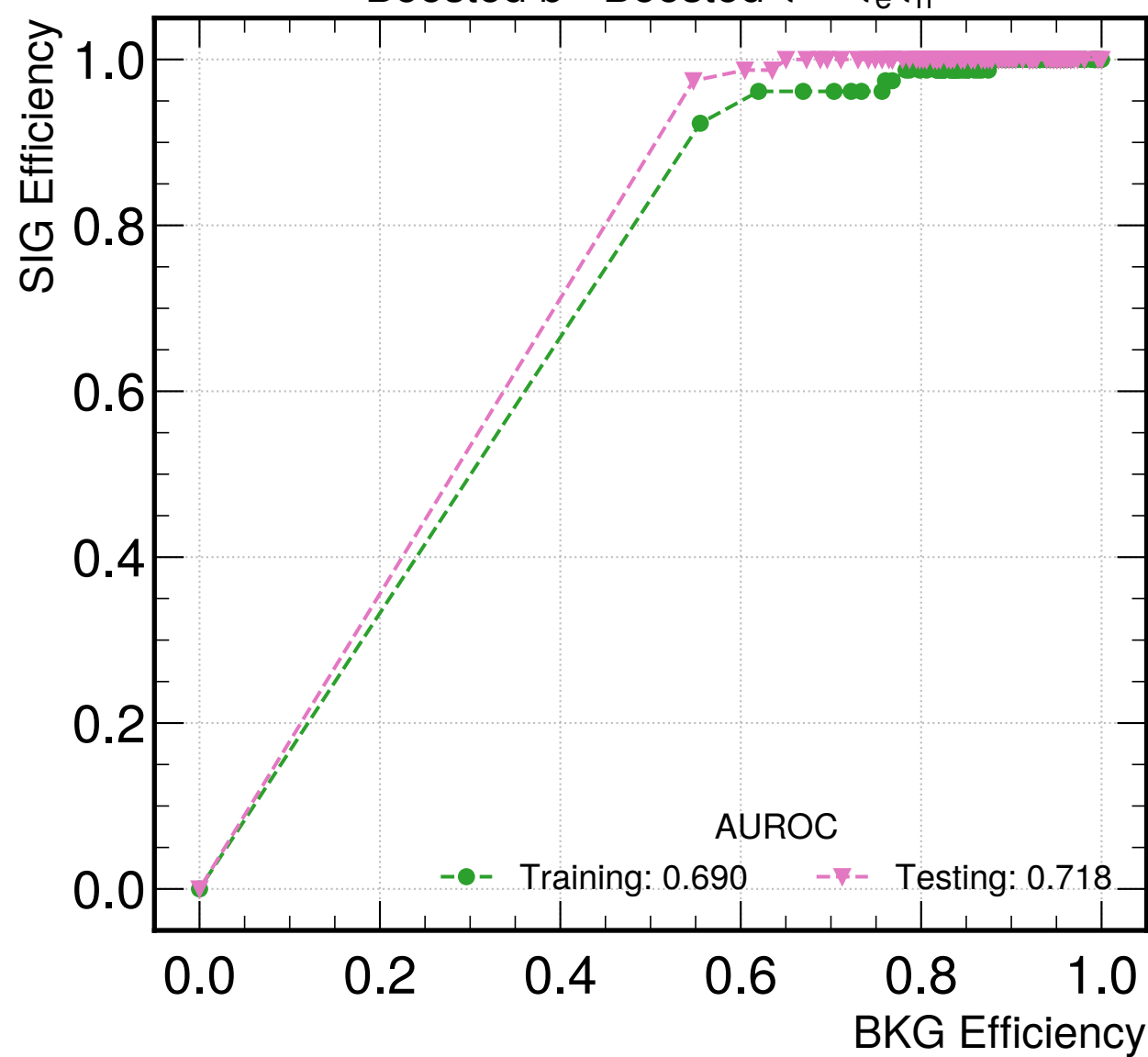
Boosted b - Boosted \tau -- \tau_e\tau_h
