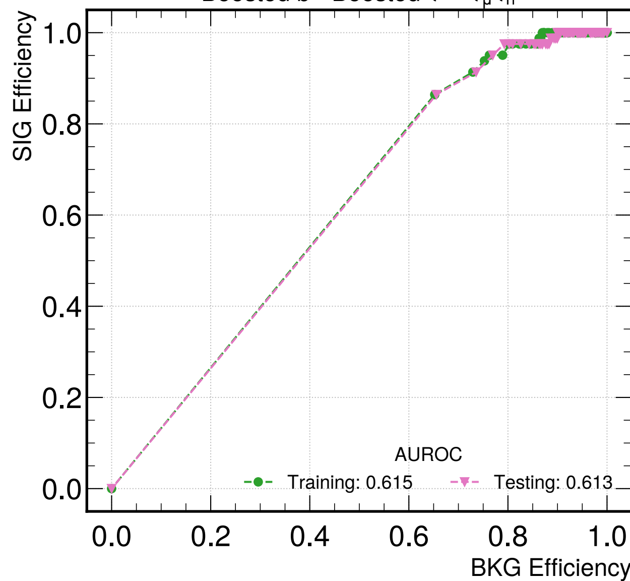
Boosted b - Boosted \tau -- \tau_\mu\tau_h
