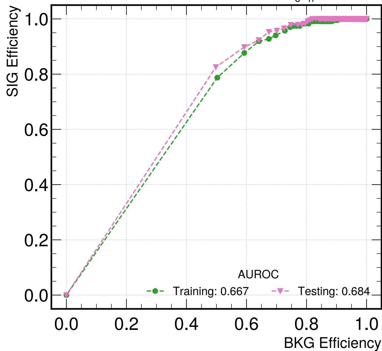
Boosted b - Resolved \tau -- \tau_e\tau_h
