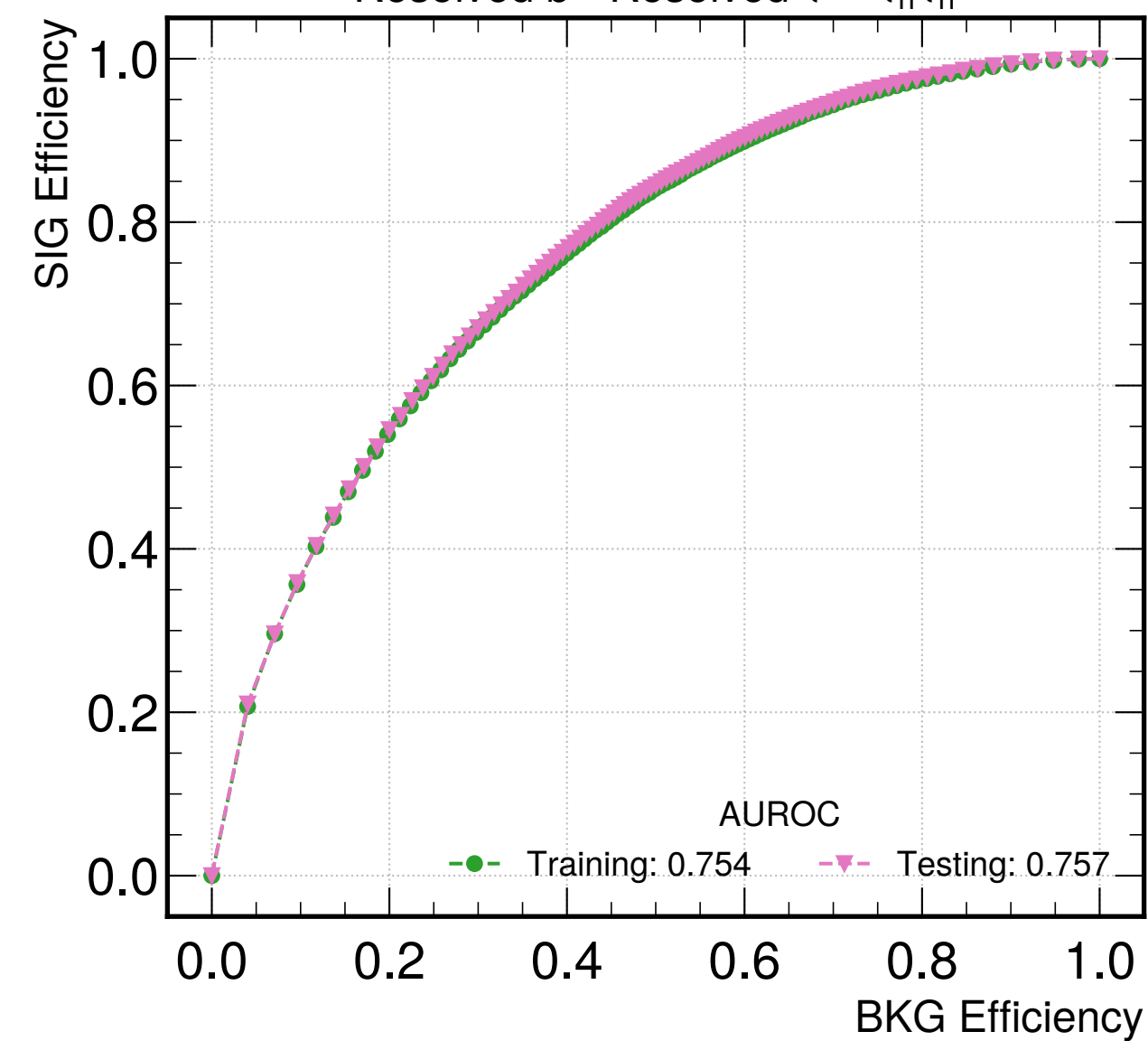
Resolved b - Resolved \tau -- \tau_h\tau_h
