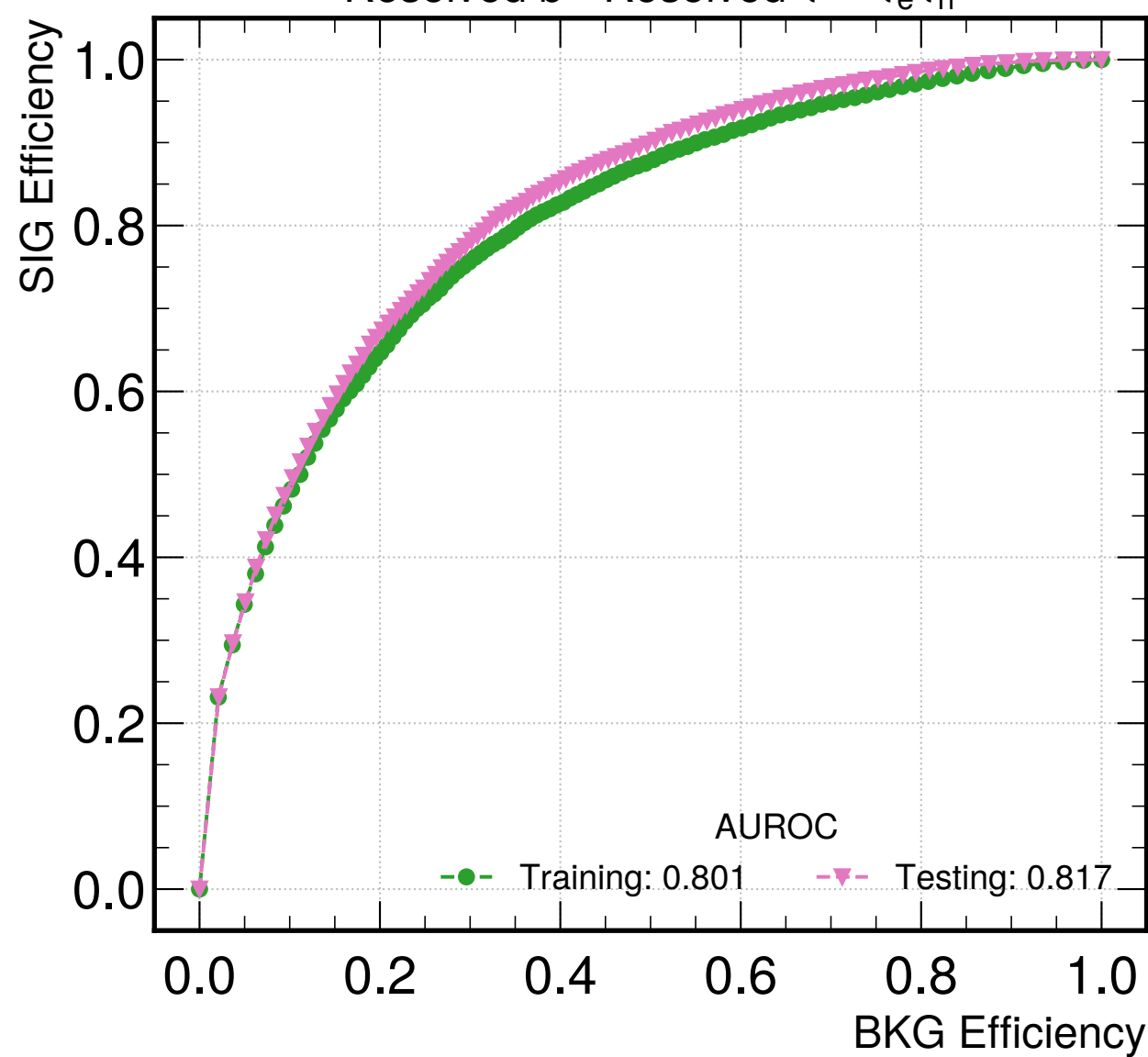
Resolved b - Resolved \tau -- \tau_e\tau_h
